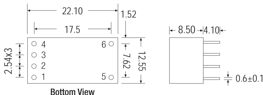
Package A: RCD-24-XXX – Style and pinning (mm)
